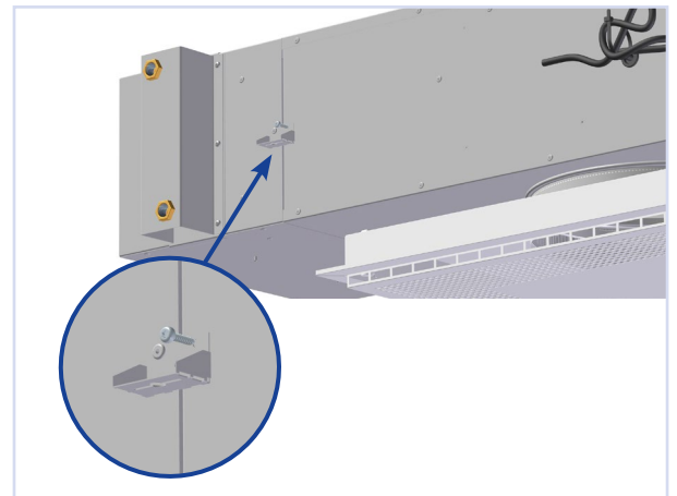
Figure 4, Mounting.
