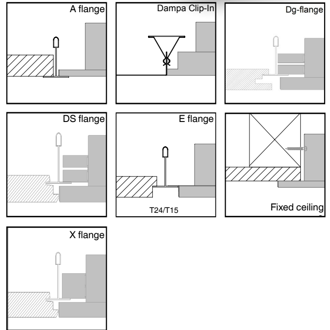
Figure 4, Mounting.
