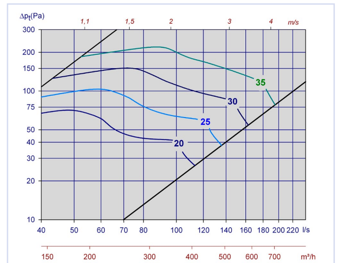
Diagram 4, Orion PTV with Sirius Comfort 250
