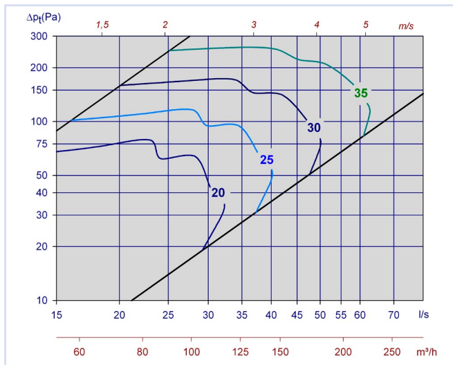
Diagram 1, Orion PTV with Sirius Comfort 125
