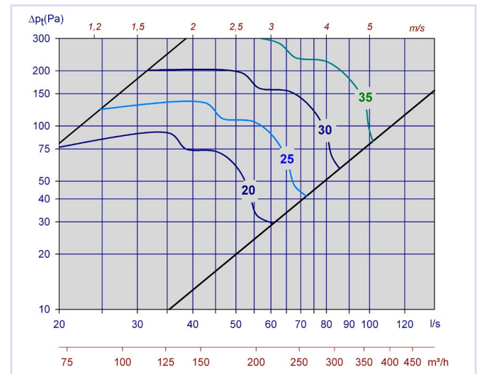
Diagram 2, Orion PTV with Sirius Comfort 160
