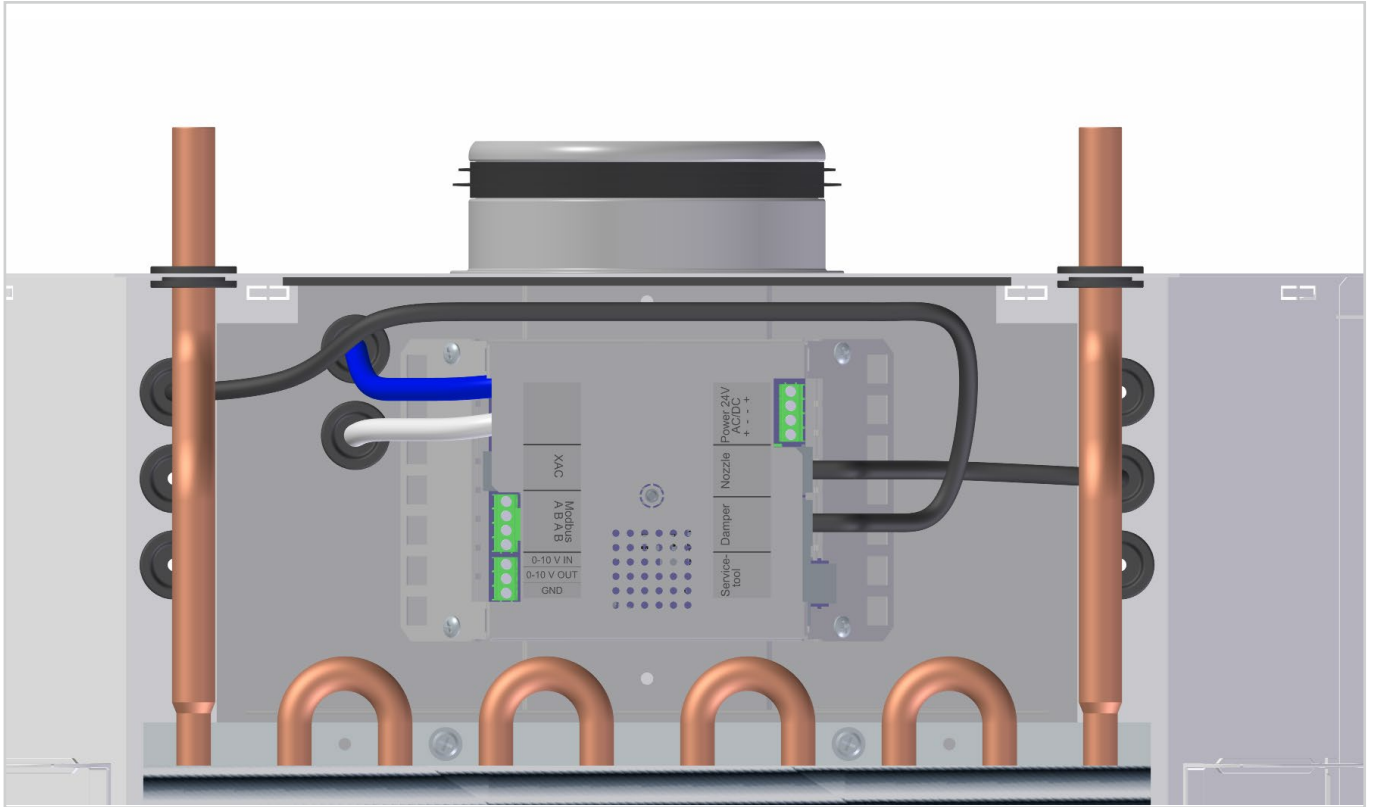
Figure 13, Regulator
