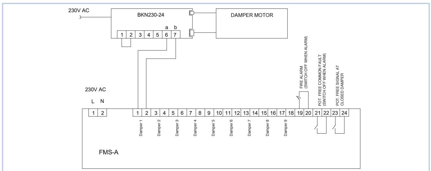
Figure 1, electrical installation
