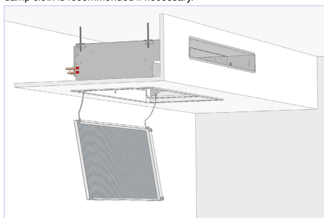
Figure 13, maintenance
