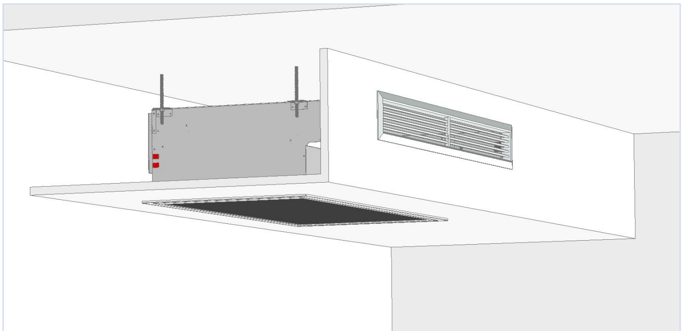
Figure 9. Mounting
