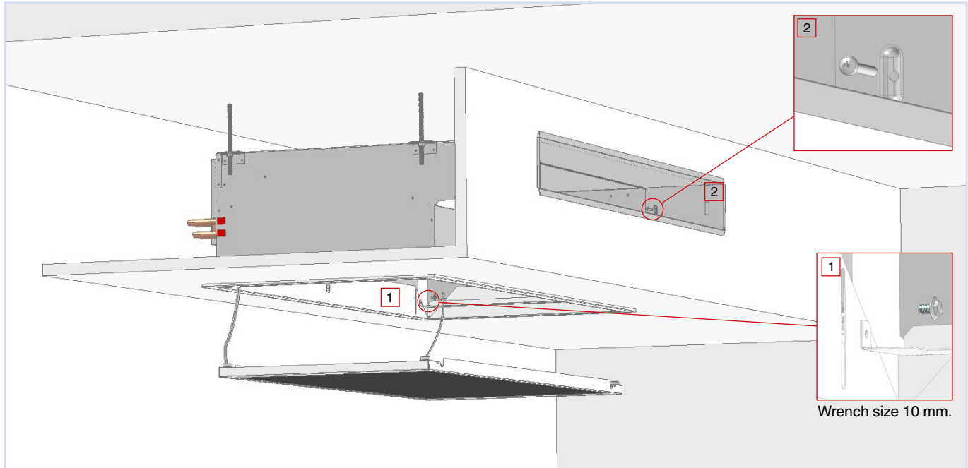
Figure 8. Mounting. When the baffle is secured to the ceiling with threaded rods, the frame for the secondary grille can be fastened back to the rim using four screws. The grille is clamped up to the suspended ceiling and the screws are tightened (1). Click secondary grille in place. Telescopic frame for front grille is attached to the short sides of the frame with mounting screws(2).
