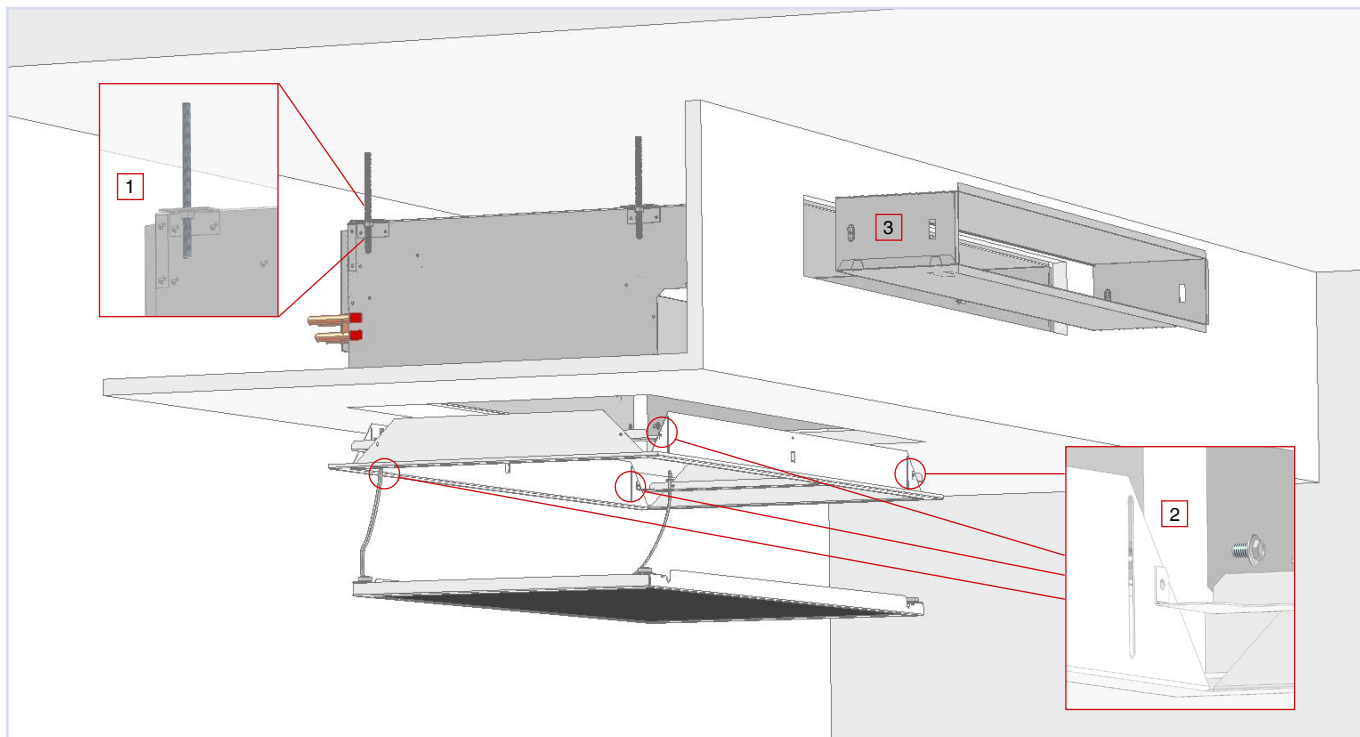
Figure 7. Installation.
