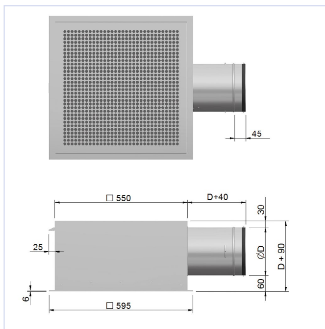
Figur 3, Orion-ATV- S (Ø160 - 315) m/spjeld
