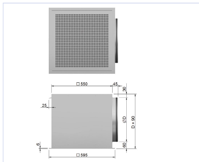
Figur 4, Orion-ATV- S Ø400 u/spjeld.
