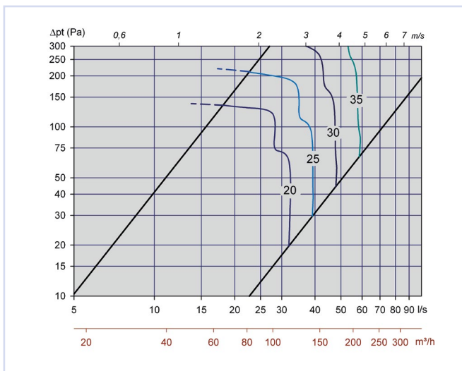
Diagram 9, Pegasus Opus 125-B
