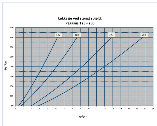
Figur 7, Lekkasmengde Pegasus
