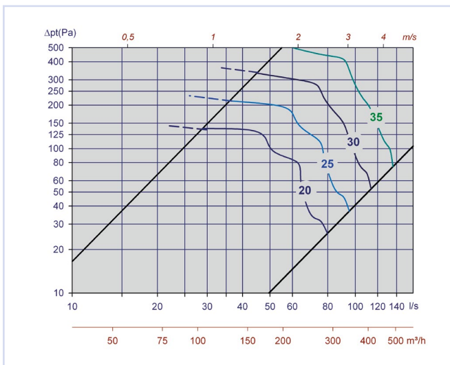
Diagram 7, Pegasus LÖV 200-S
