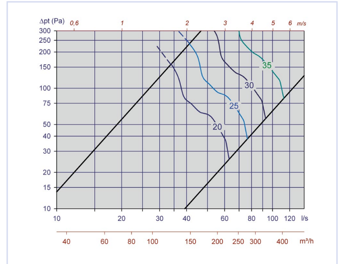
Diagram 6, Pegasus LÖV 160-S
