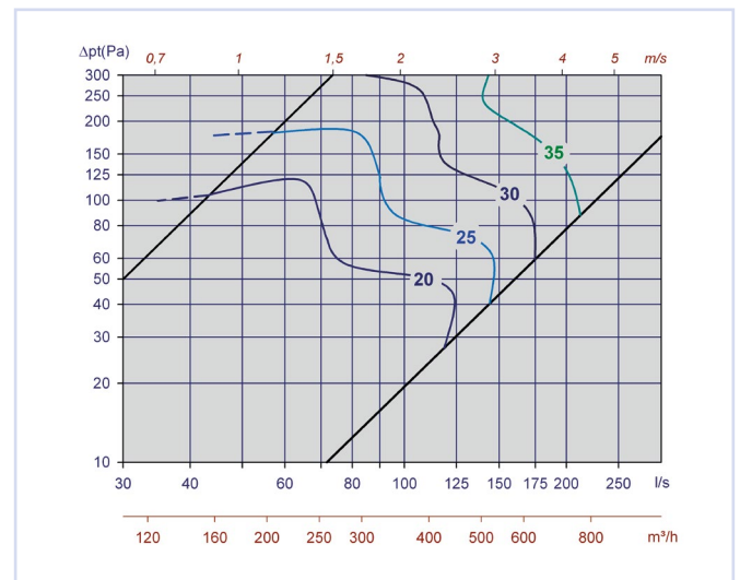
Diagram 8, Pegasus LÖV 250-S
