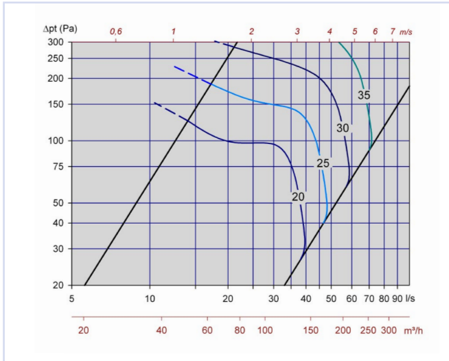
Diagram 5, Pegasus LÖV 125-S
